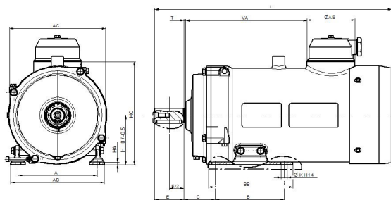
Foot-mounted B3
